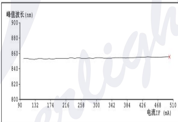
Spectral wavelength
