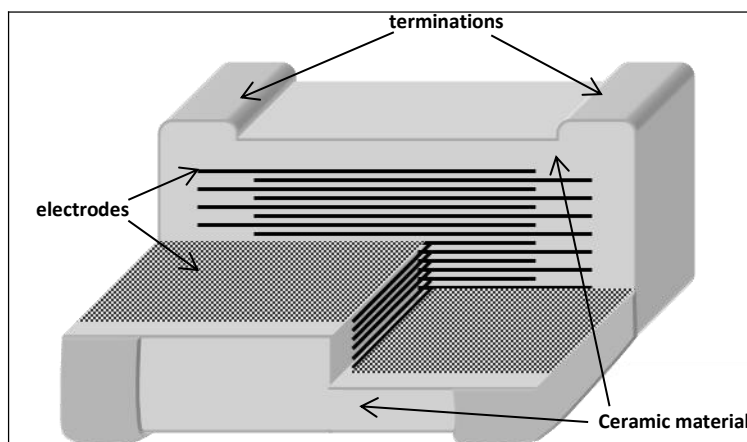
Fig. 1 Surface mounted multilayer ceramic capacitor construction
