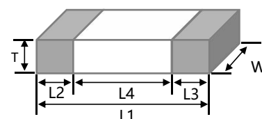
Fig. 2 Surface mounted multilayer ceramic capacitor dimension
