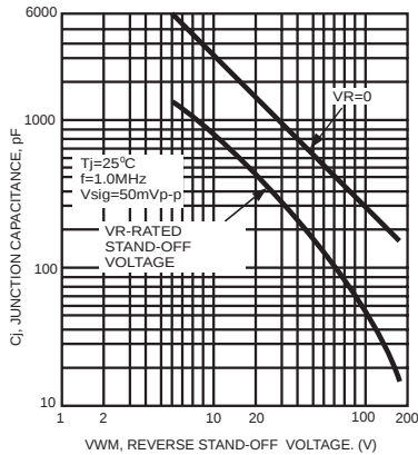
FIG.5- TYPICAL JUNCTION CAPACITANCE
