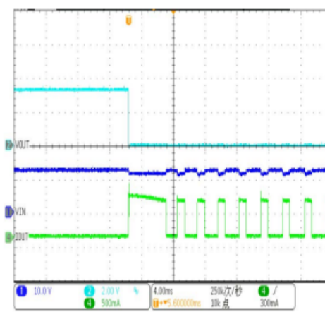
Power-on short
