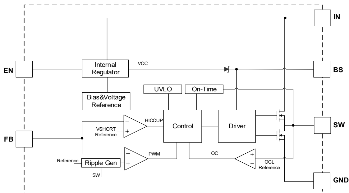
Block Diagram
