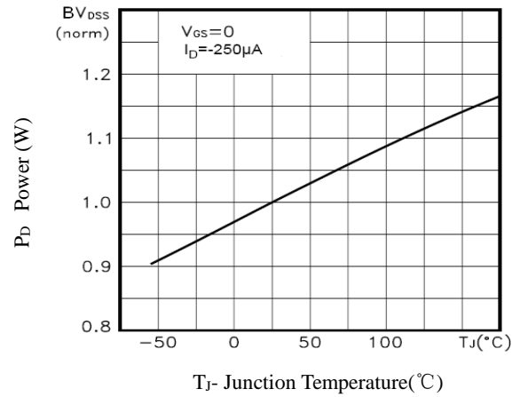
Figure 23. Power Dissipation
