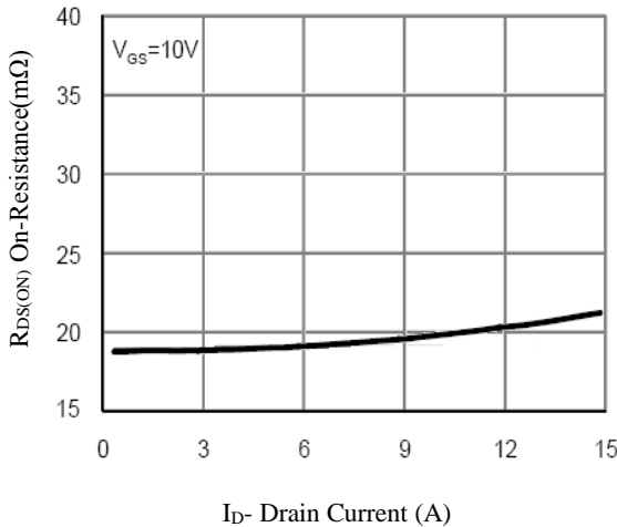
Figure 7. Drain-Source On-Resistance
