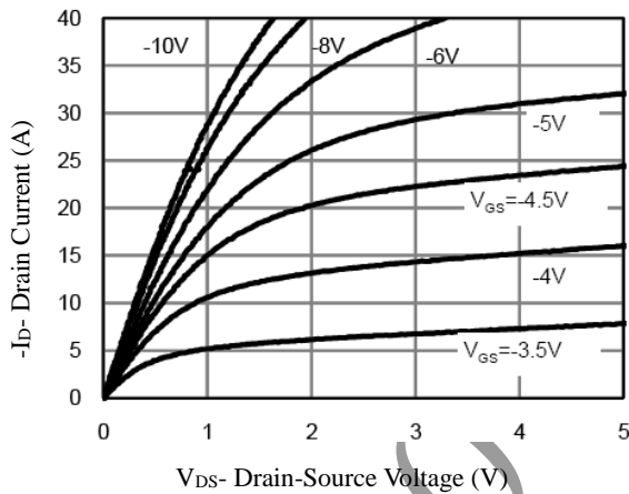
Figure 16. Output Characteristics
