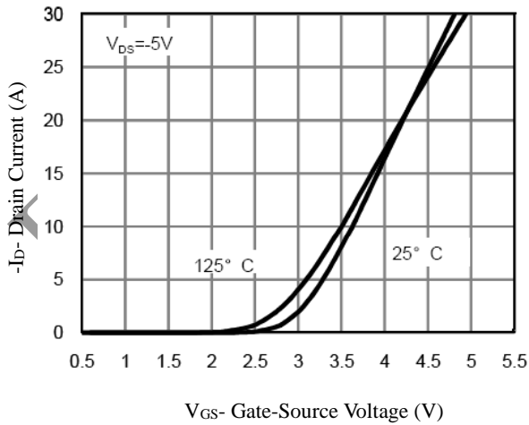
Figure 18. Transfer Characteristics
