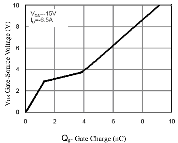
Figure 19. Gate Charge
