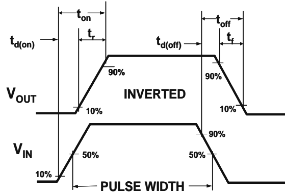
Figure 4. Switching Waveforms
