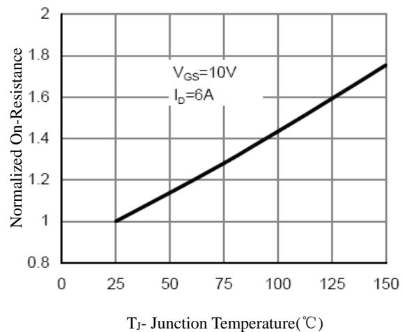
Figure 8. Drain-Source On-Resistance
