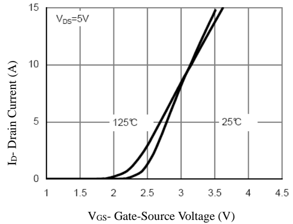
Figure 6. Transfer Characteristics
