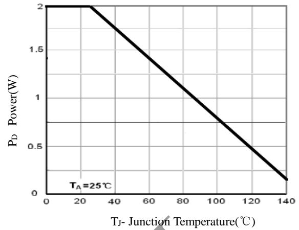
Figure 10. Power Dissipation
