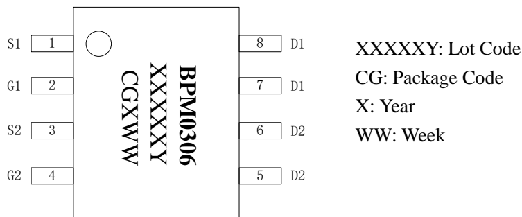
Figure 2. Pin Configuration
