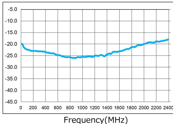
Output 2 Return Loss (Pin3)
