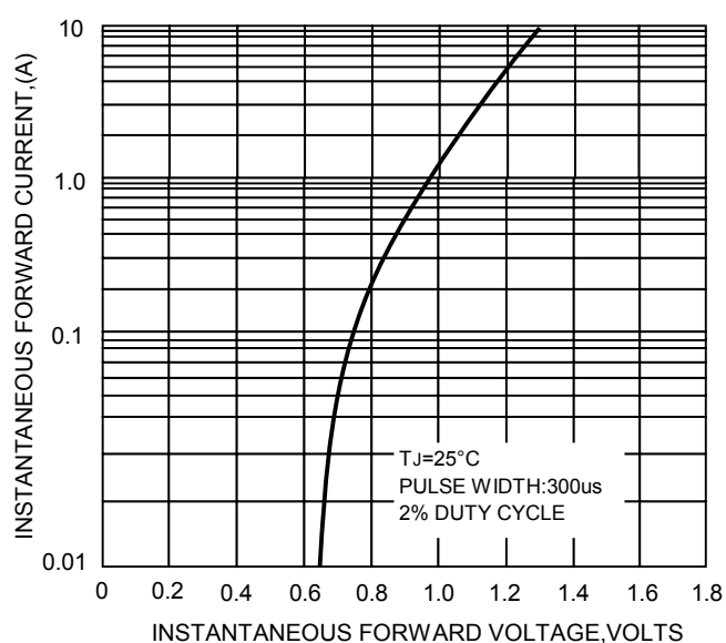
FIG.4-TYPICAL FORWARD CHARACTERISTICS
