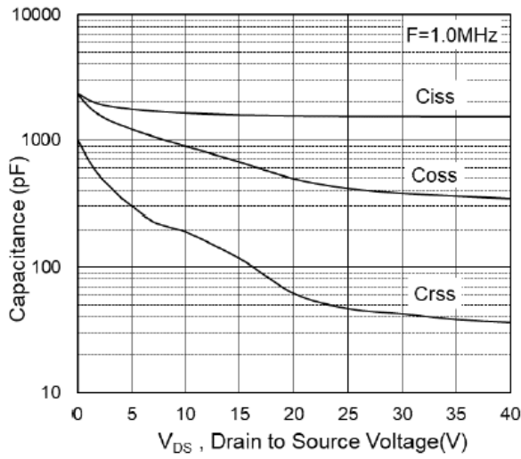
Fig.7 Capacitance
