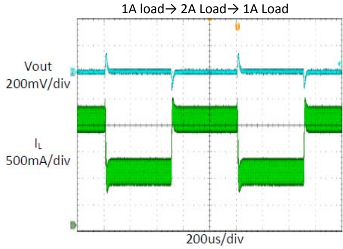
Load Transient
