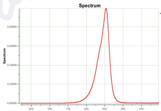
Spectral wavelength
