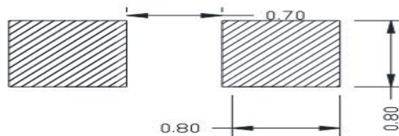
Recommended Soldering Pattern (建议焊盘尺寸图)
