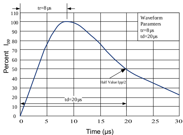
Figure 5: Pulse Waveform
