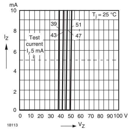
Fig. 16 - Breakdown Characteristics
