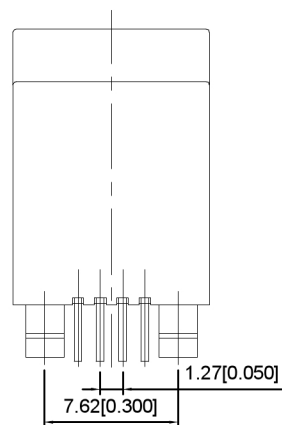
BOTTOM VIEW
