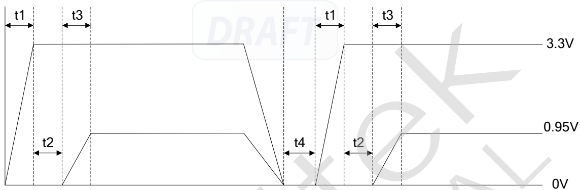
Figure 6. Power Sequence
