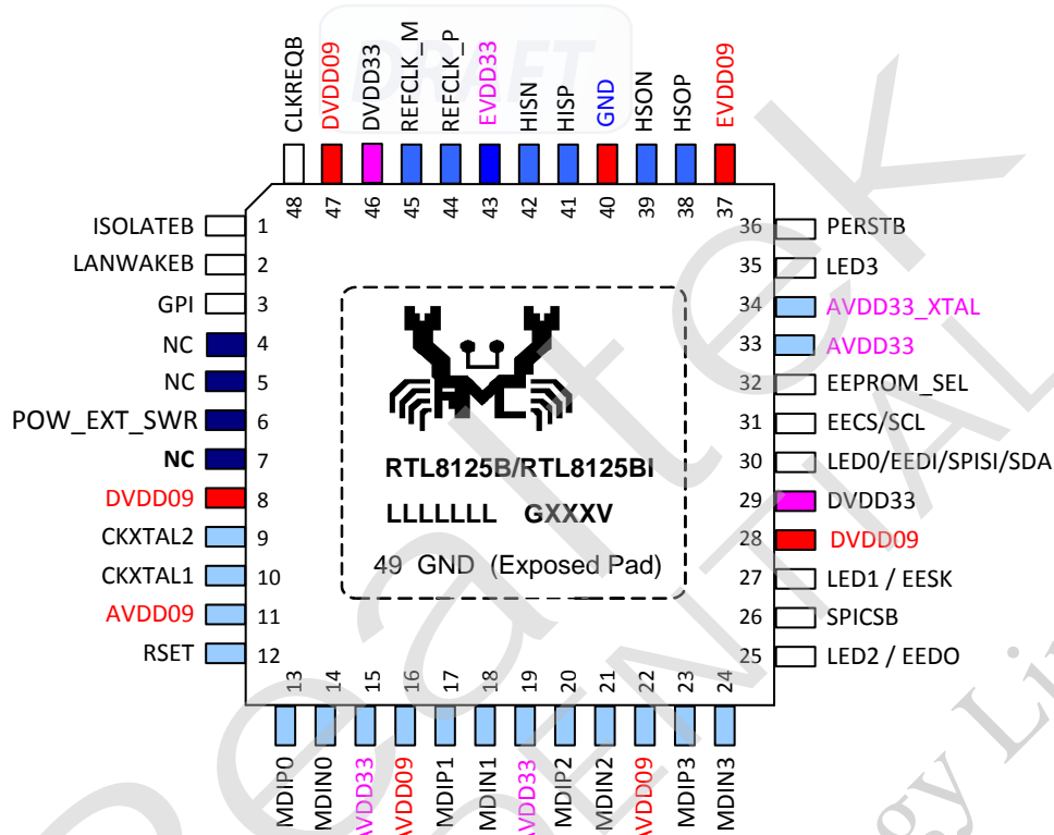
Figure 2. RTL8125B/RTL8125BI Pin Assignments
