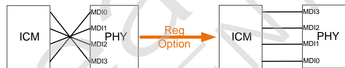
Figure 5. MDI SWAP
