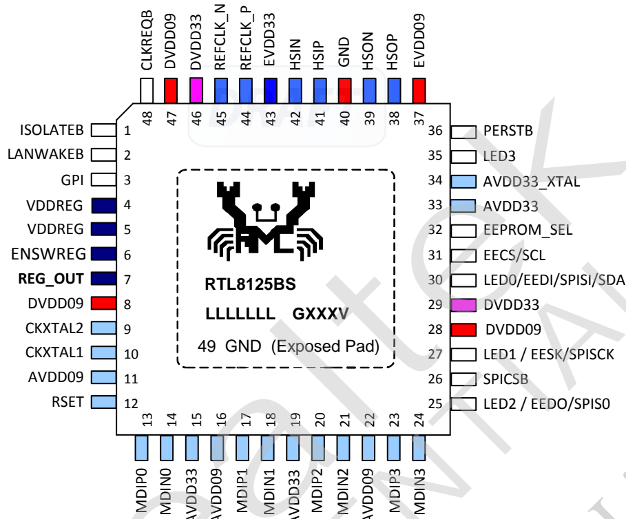
Figure 3. RTL8125BS Pin Assignments
