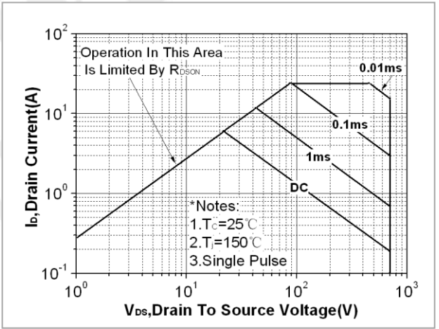
Fig. 12. Maximum safe operating area (TO-251&TO-251N)
