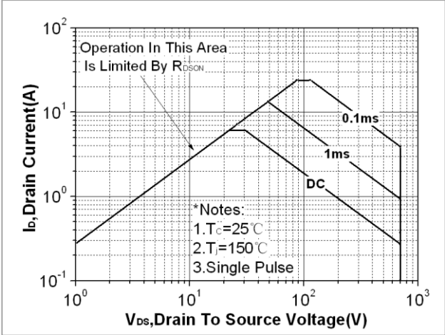
Fig. 14. Maximum safe operating area(TO-220)
