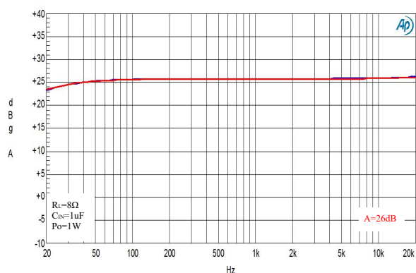
Frequency Response, 12V, 8Ω load (BTL)
