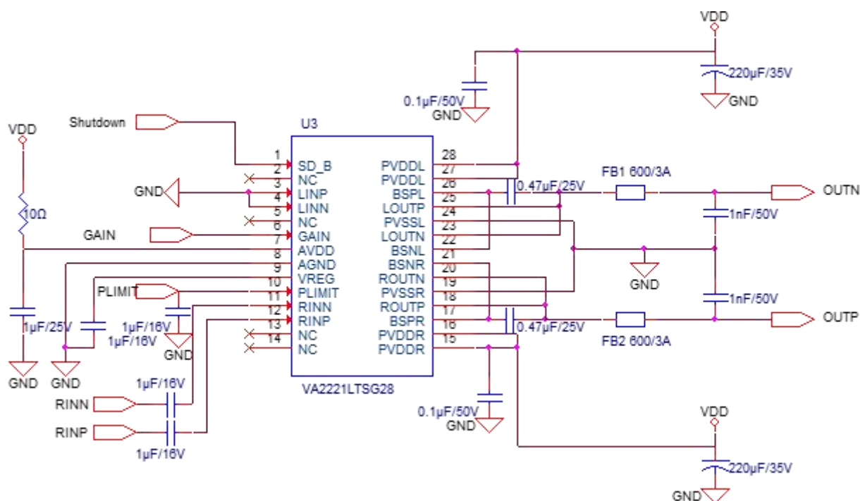
Figure 8. VA2221L Mono Reference Application with Ferrite Bead
