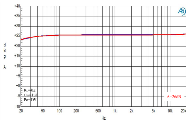
Frequency Response, 12V, 4Ω load (BTL)
