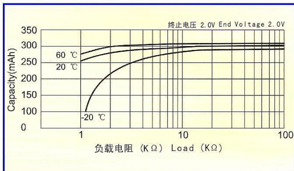
Load-capacity
