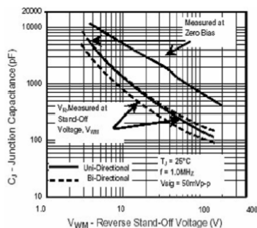
Fig4. Typical Junction
