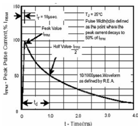
Fig3. Pulse Waveform
