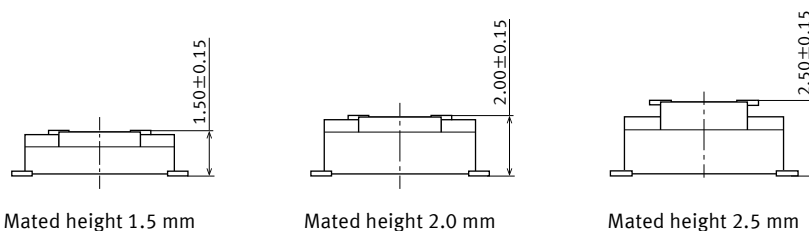
Mated height 1.5 mm
