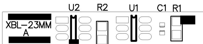
TOP SILKSCREEN
