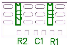
TOP SILKSCREEN
