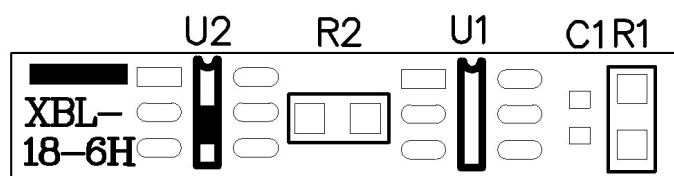
TOP SILKSCREEN
