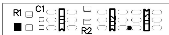
TOP SILKSCREEN
