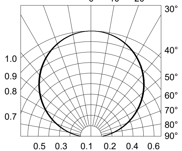
Fig.6-Radiation Diagram T_a=25^{\circ}\text{C}
