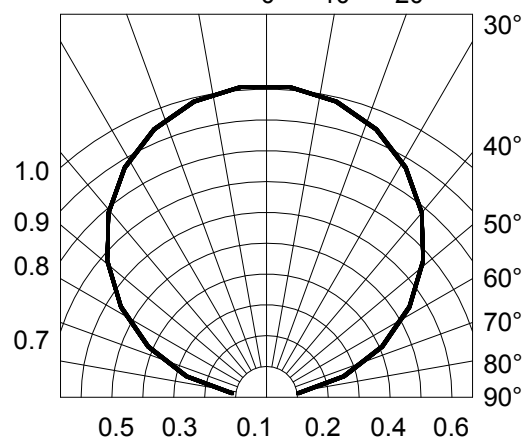
Fig.6-Radiation Diagram Ta=25°C
