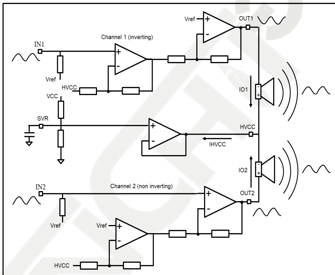
Figure 5 Amplifier Structure
