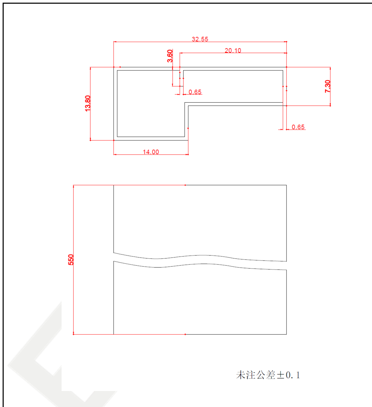
Figure 8 Tube Packing Information
