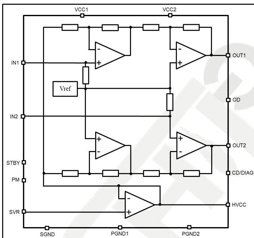
Figure 1 Block diagram
