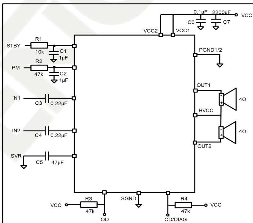
Figure 2 Application circuit
