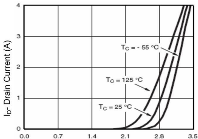
Figure 7 Transfer Characteristics
