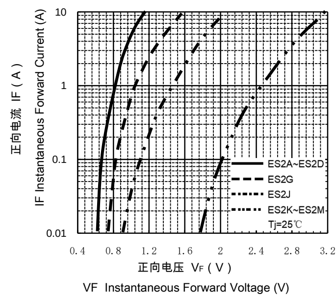
正向特性曲线 ( 典型值 ) TYPICAL FORWARD CHARACTERISTIC
