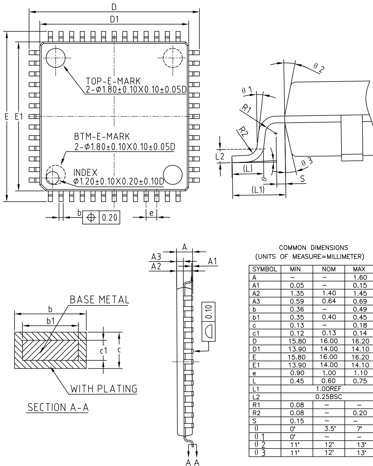
封装示意图 (LQFP52 14mm*14mm)
