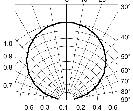
Fig.6-Radiation Diagram
