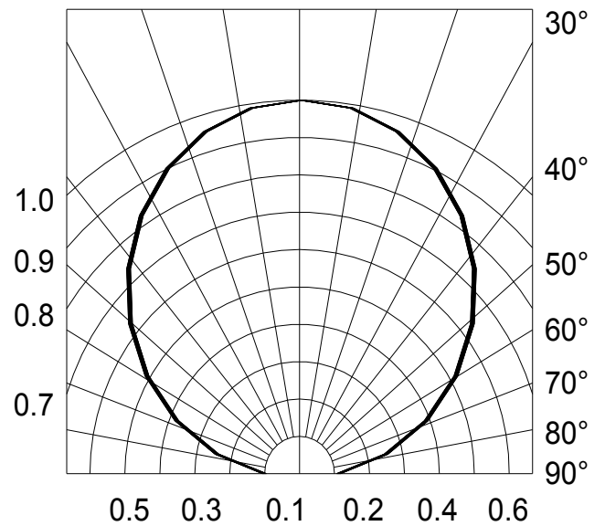
Fig.6-Radiation Diagram Ta=25°C
