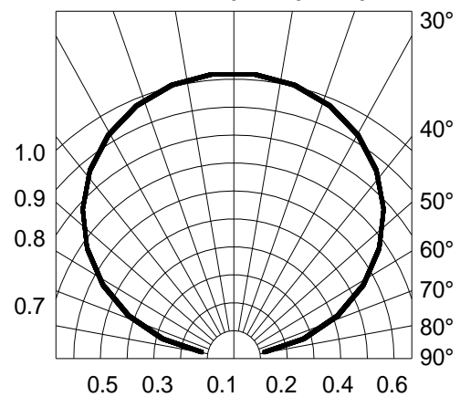
Fig.6-Radiation Diagram Ta=25°C
