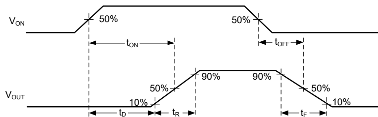
Figure 3. Timing Waveforms
