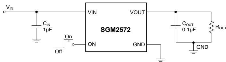
Figure 2. Test Circuit
