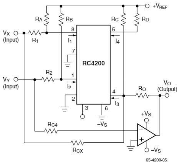
Figure 4. Extended Range Multiplier
