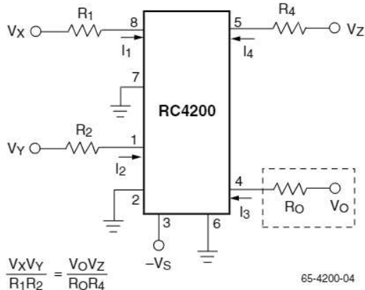
Figure 3. Voltage Multiplier/Divider
