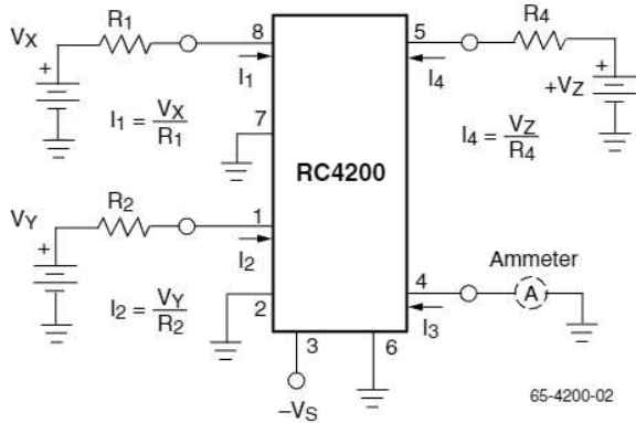
Figure 1. Current Multiplier/Divider
