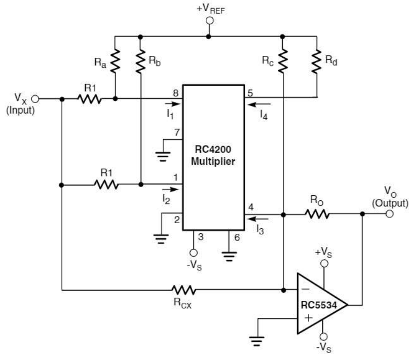
Figure 10. Squaring Circuit
