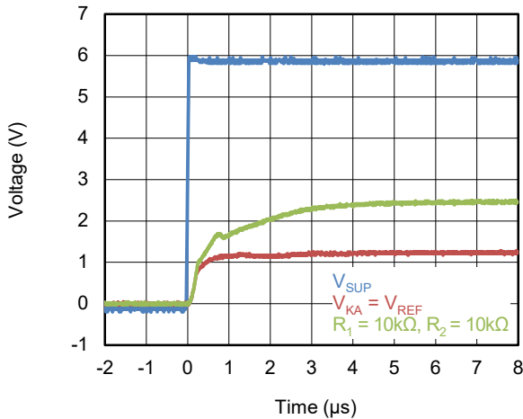
Figure 8. SGM431V Start-Up Response
