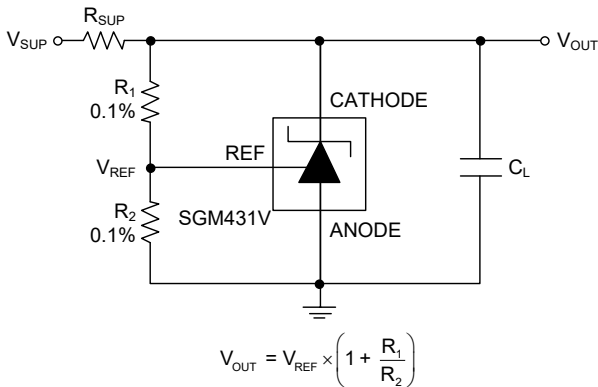
Figure 6. Shunt Regulator Schematic
