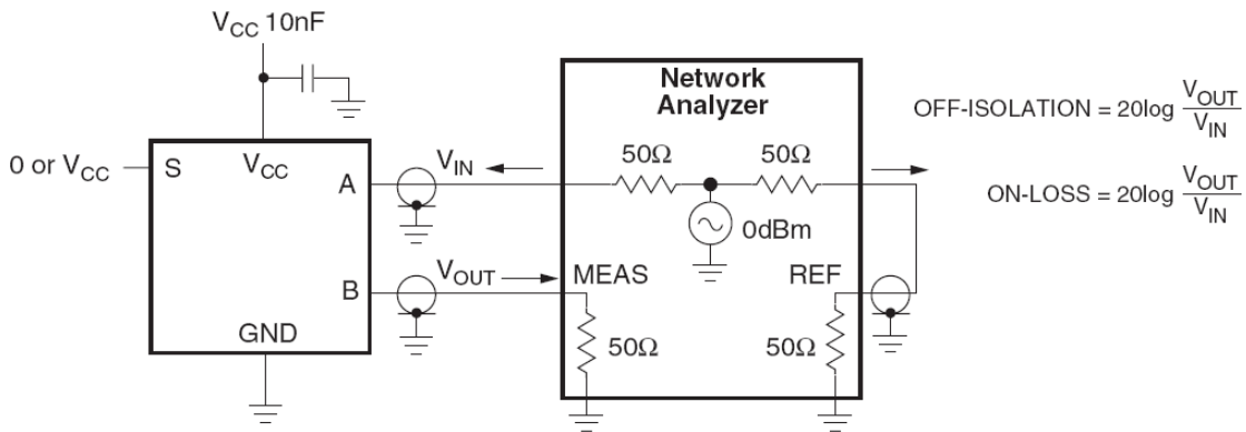
Figure 9. Off Isolation
