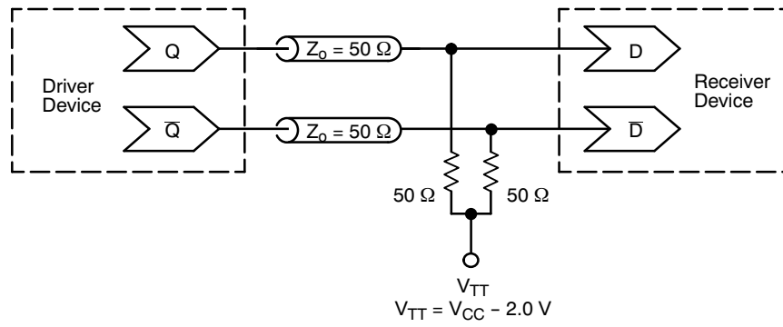
Figure 15. Typical Termination for Output Driver and Device Evaluation (See Application Note AND8020/D – Termination of ECL Logic Devices.)
