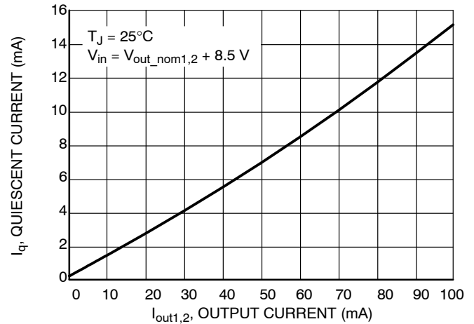
Figure 12. Quiescent Current vs. Output Current (High Load)
