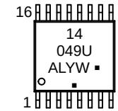
TSSOP-16 DT SUFFIX CASE 948F
