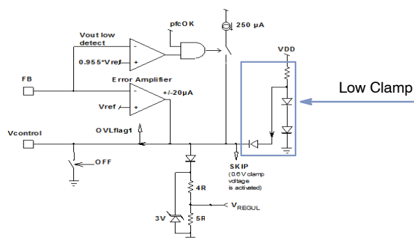
Figure 21. V_{\text{CONTROL}} Low Clamp
