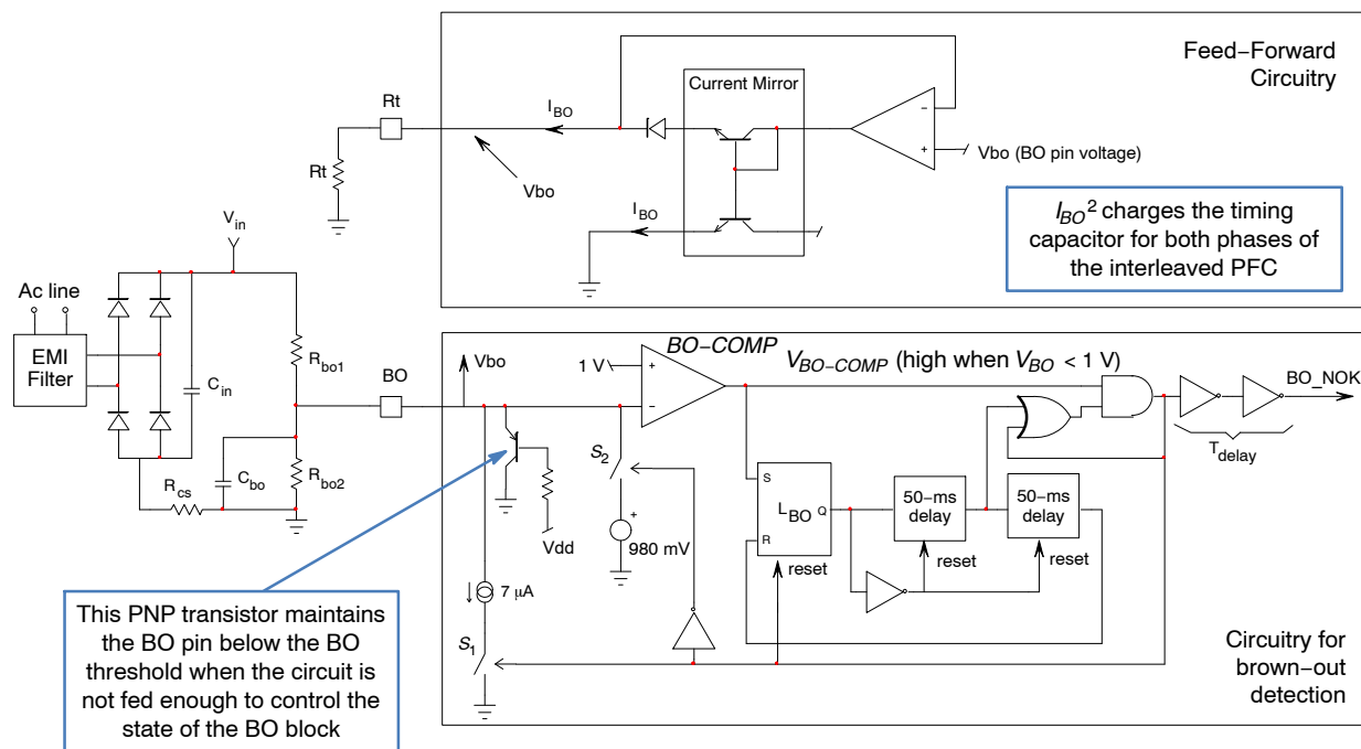
Figure 22. Brown-out Block
