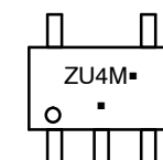
SC-88A CASE 419A-02
