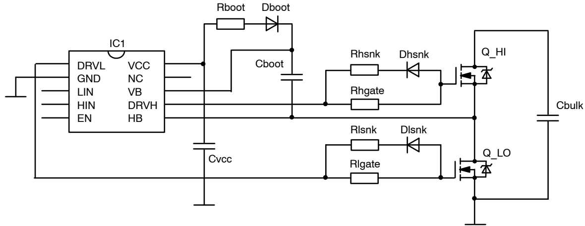
Figure 48. Recommended Schematic
