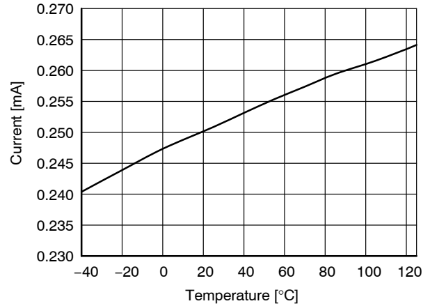
Figure 13. I_{CC1 \text{ no load}} vs. Temperature
