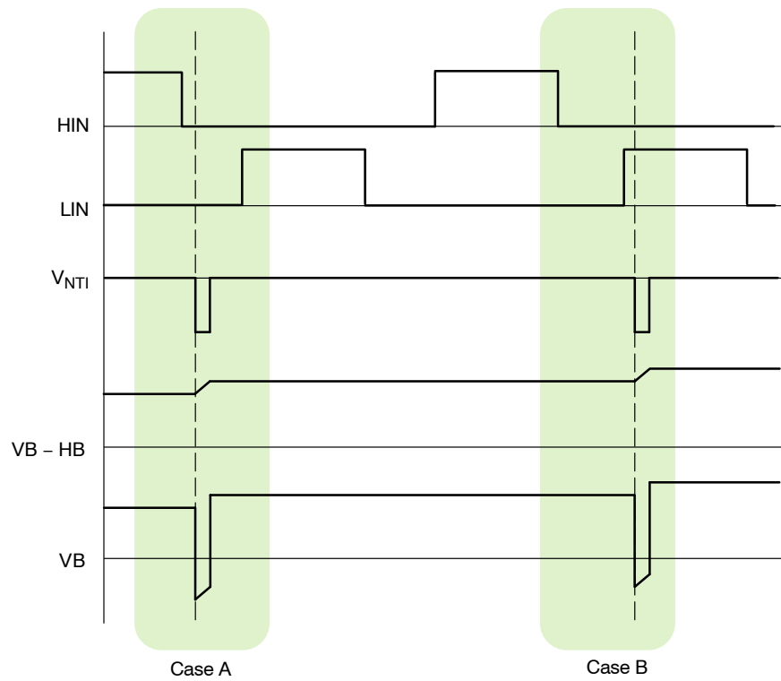
Figure 46. Timing Diagram
