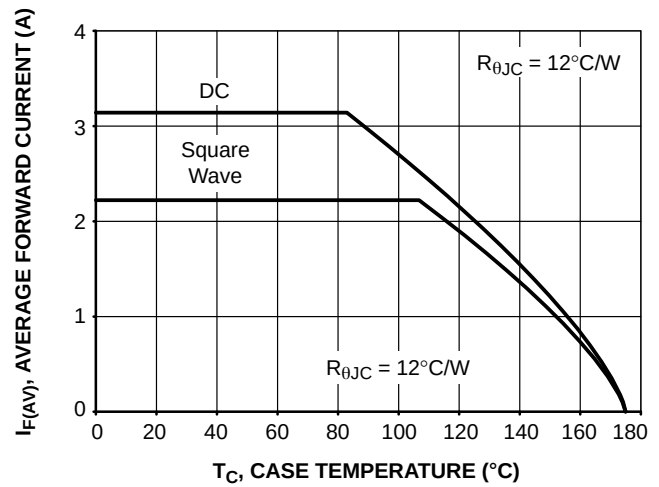
Figure 6. Current Derating
