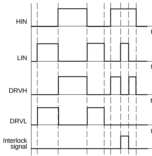
Figure 43. Interlock Timing Diagram, NCV51513xA
