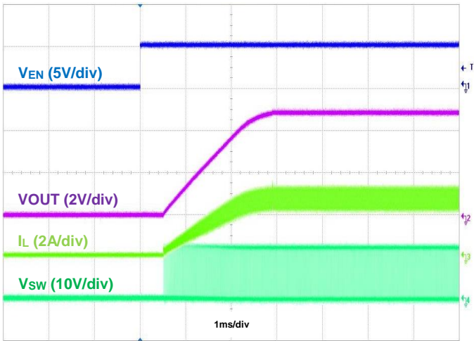
Figure 10. Startup Using EN, I_{OUT} = 3\text{A}
