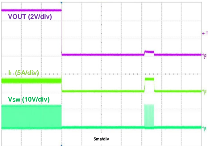
Figure 12. Output Short Protection, I_{OUT} = 3\text{A}
