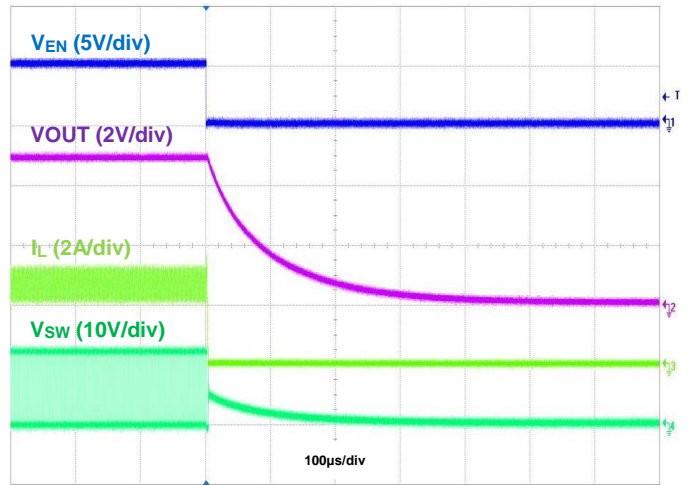
Figure 11. Shutdown Using EN, I_{OUT} = 3\text{A}
