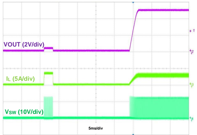
Figure 13. Output Short Recovery, I_{OUT} = 3\text{A}
