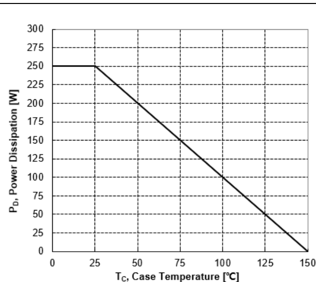
Figure 2. Maximum Power Dissipation vs Case Temperature
