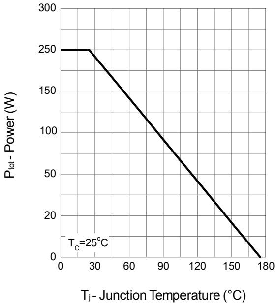
Power Dissipation
