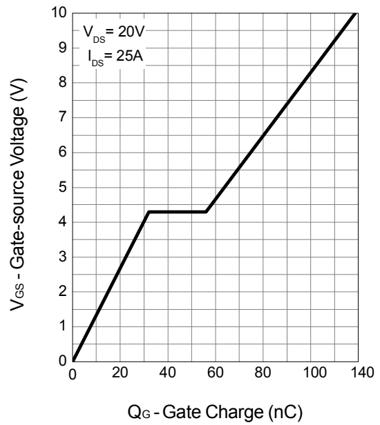
Gate Charge
