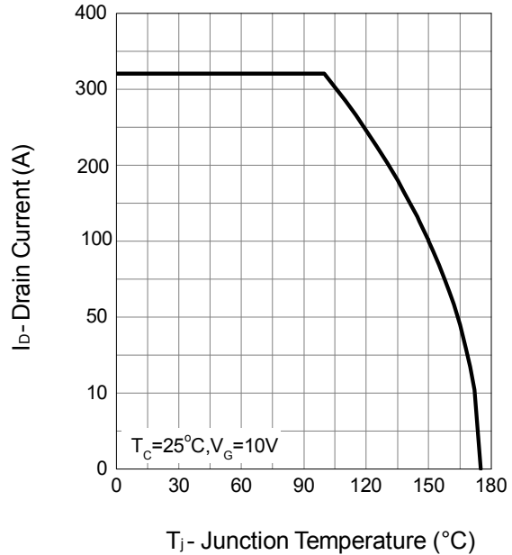
Drain Current
