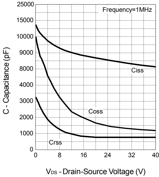
Capacitance
