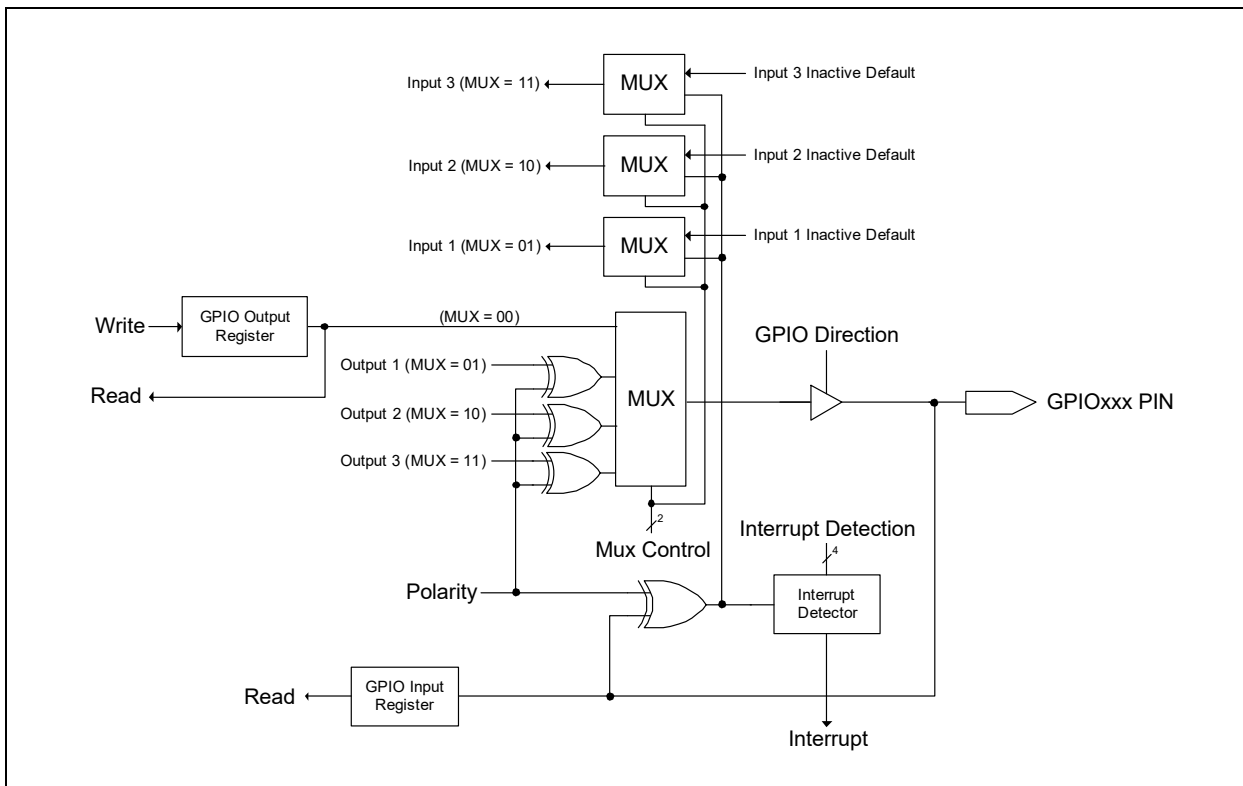
FIGURE 11-1: GPIO BLOCK DIAGRAM
