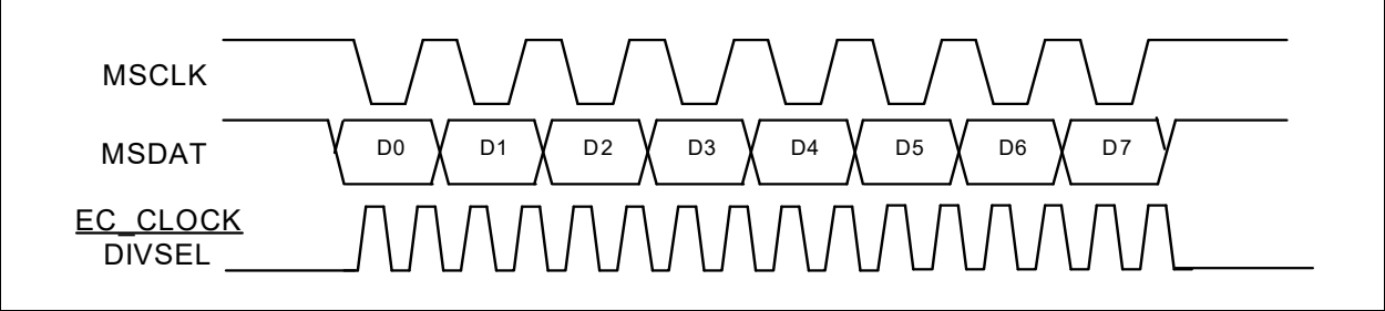
FIGURE 30-3: DATA TRANSFER
