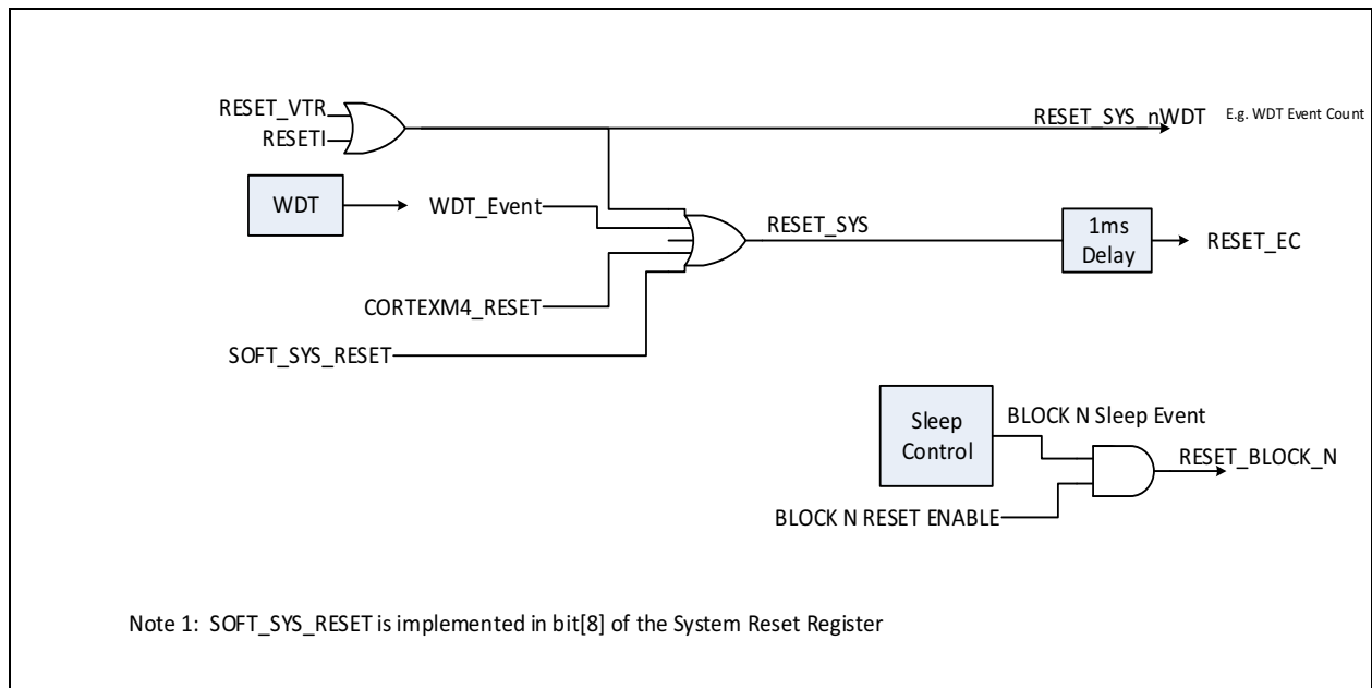
FIGURE 5-4: RESETS BLOCK DIAGRAM (CEC1702)
