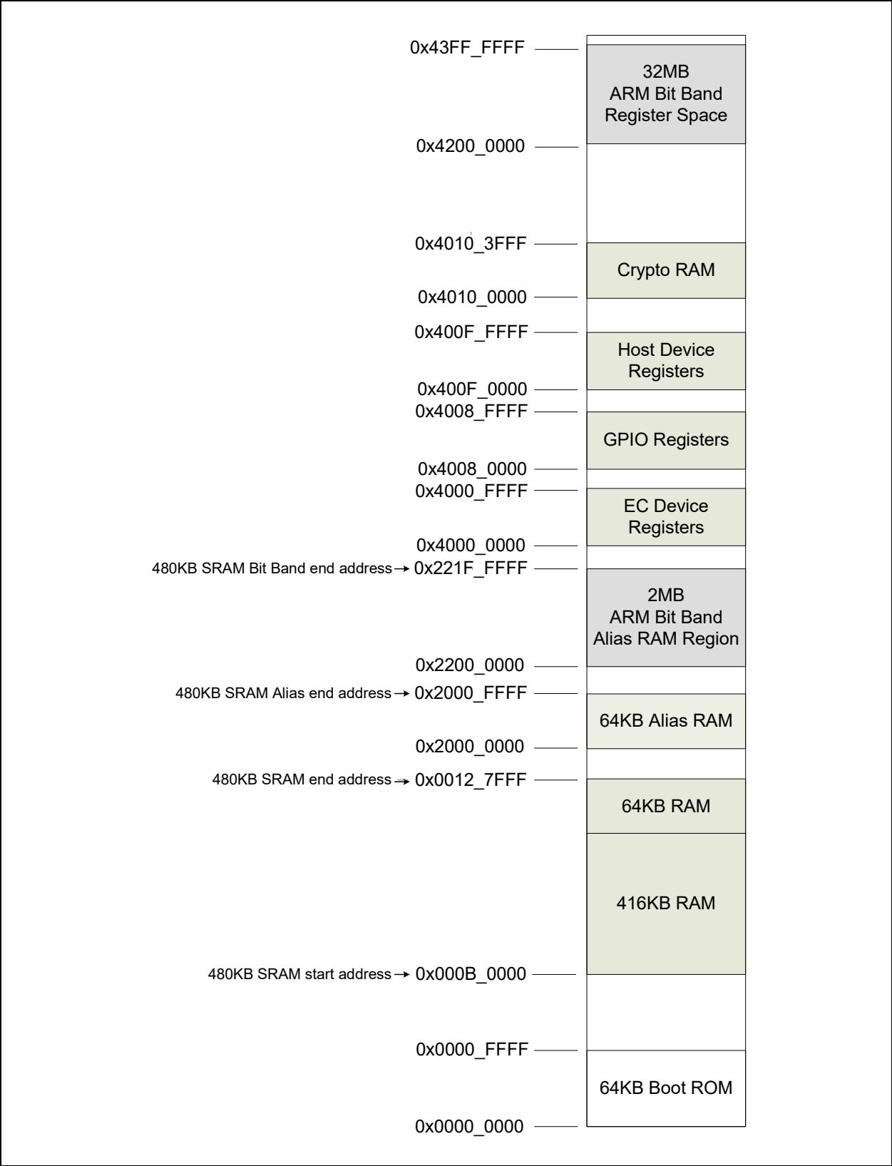
FIGURE 6-1: MEMORY LAYOUT
