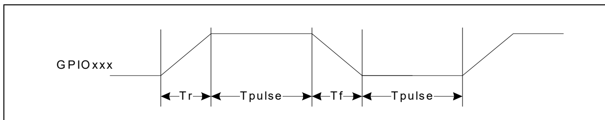
FIGURE 39-6: GPIO TIMING
